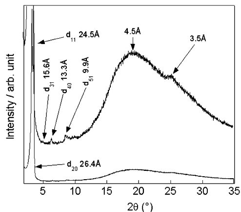
Fig. 4 X-Ray diffraction patterns of 3F at 205 °C.
