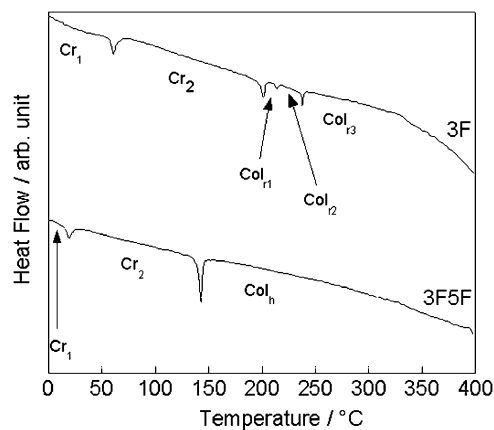
Fig. 3 DSC curves of 3F and 3F5F (heating rate 5 \text{ °C min}^{-1} ). Cr: Crystal, \text{Col}_r : rectangular columnar phase, \text{Col}_h : hexagonal columnar phase. Iso: isotropic liquid.
