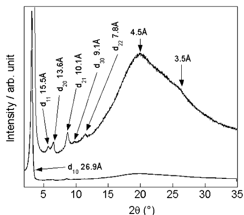
Fig. 5 X-Ray diffraction patterns of 3F5F at 160 °C.
